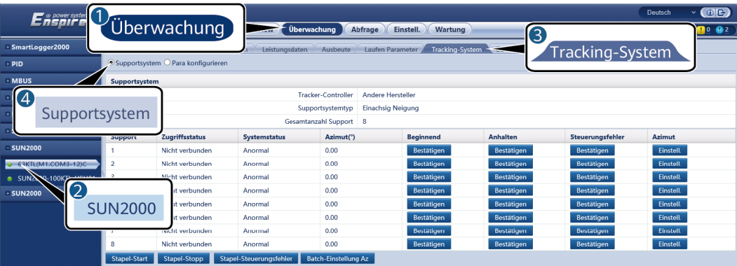
Abbildung 6-44 Supportsystem (Tracking-System)
