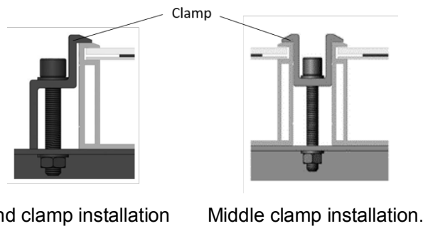
Figure 2. PV module installed with clamp fitting method
