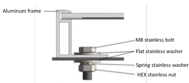
Figure 1. PV module installed with bolt fitting method.
