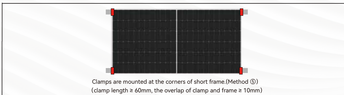
Figure 7 Mono-facial Module Installation Position
