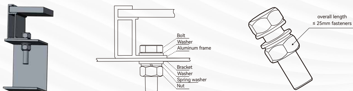
Figure 4 Bolt Installation of Modules
