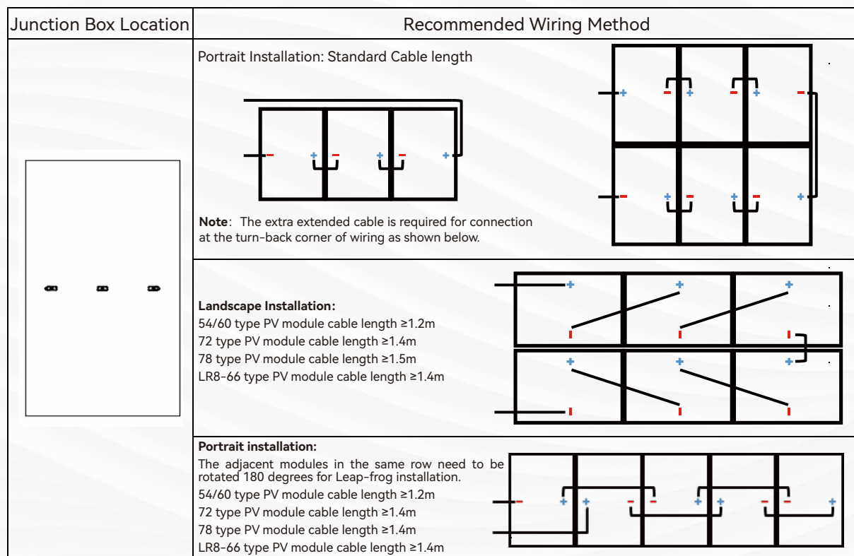
Figure2 Junction Box Style and Wiring Method
