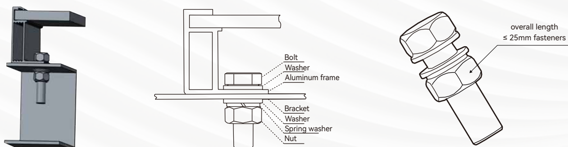
Figure 5 Bolt Installation of Modules
