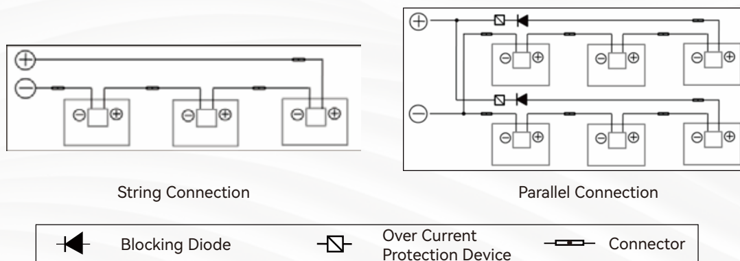
Figure 9: Series Connection and Parallel Connection Circuit Diagram
